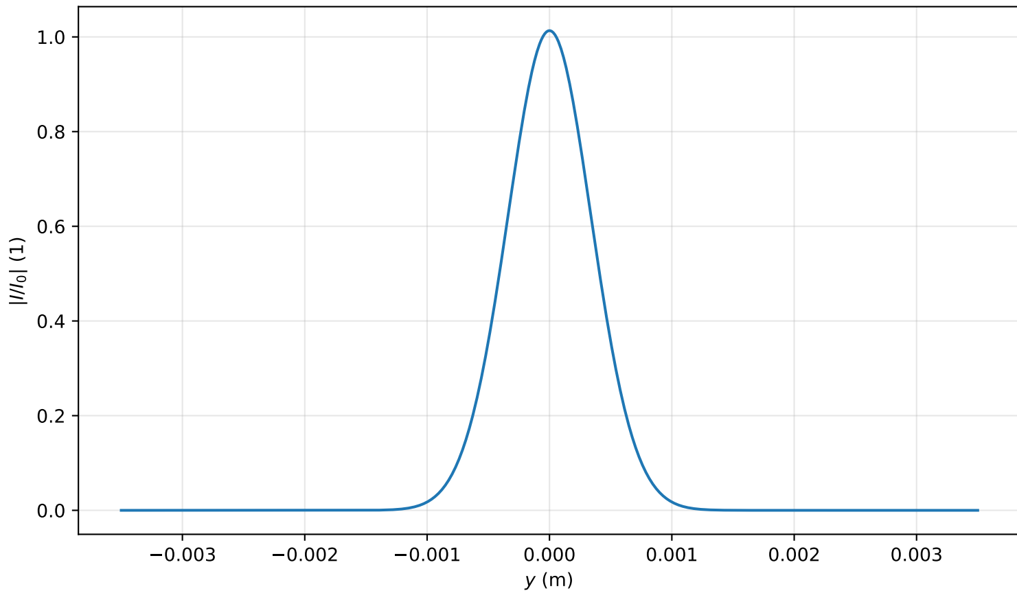
Intensity profile I(x=0, y, z=0.239)/I_0 , P_{in}=0.5P_{cr} , artificial time
